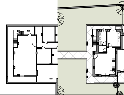
Plan piano interrato
